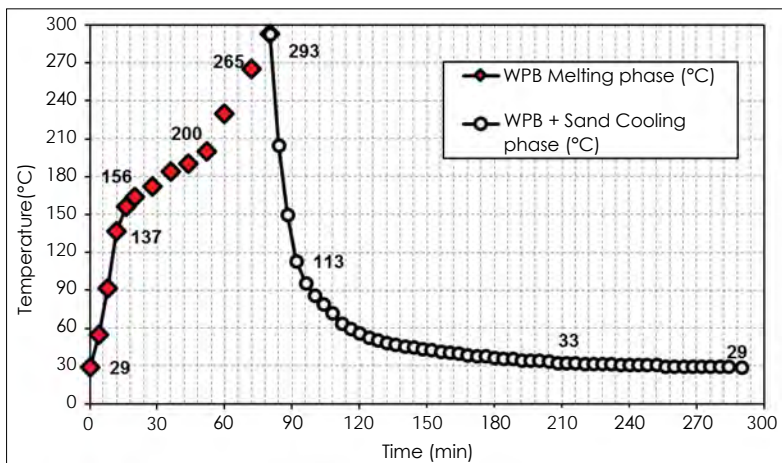
Figure 4: Recorded temperature in waste plastic bags (WPB) melting phase coupled with sand aggregates-melted plastic mix (WPB + Sand) cooling phase during the coating process
